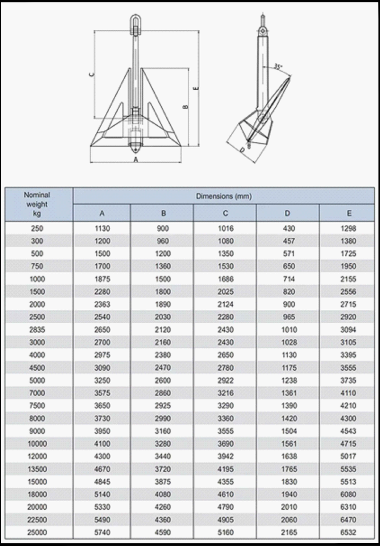
Anchor Chart details
